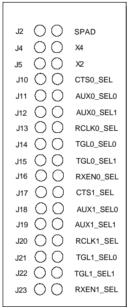
Figure 2 - Right Card Edge Jumpers
