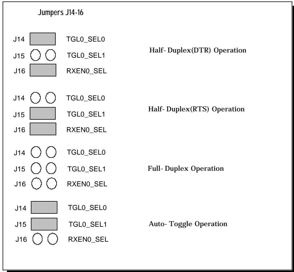
Figure 23 --- Half/full-duplex and Auto-Toggle selection
