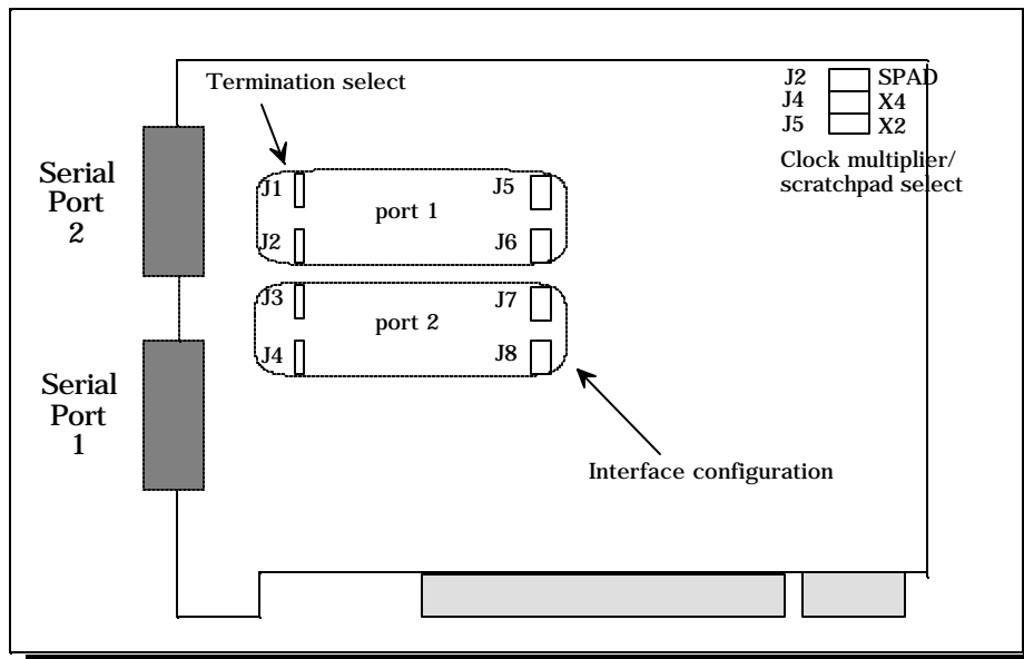
Figure 6 --- Jumper/connector locations
