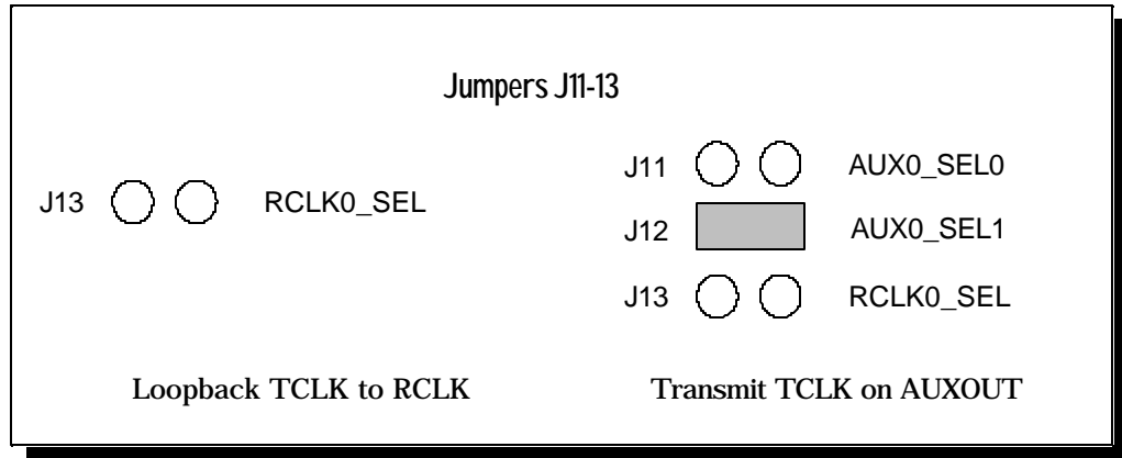
Figure 21 --- TCLK selection
