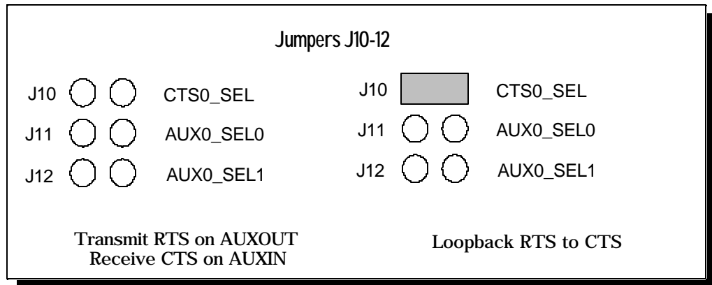
Figure 19 --- RTS/CTS selection
