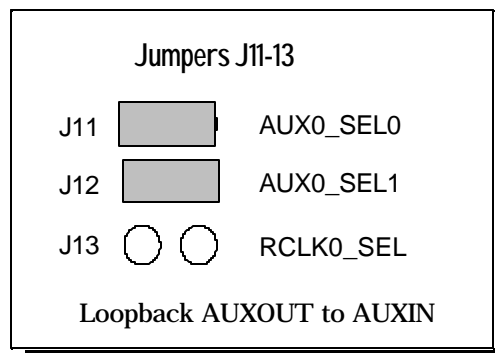
Figure 22 --- AUXIN/AUXOUT loopback
