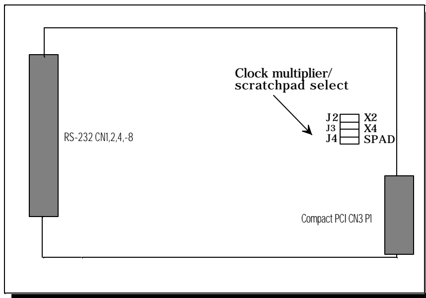
Figure 4 --- Jumper/connector locations
