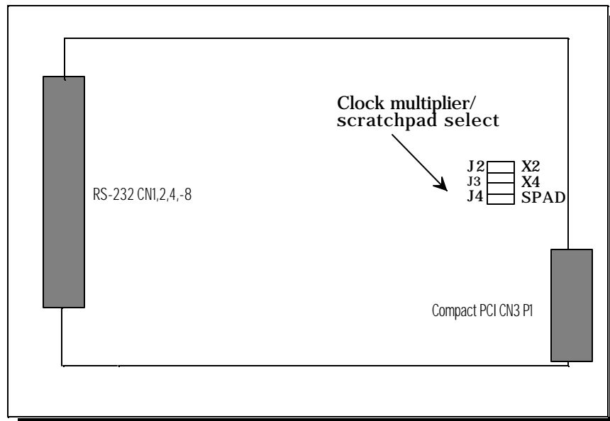
Figure 4 --- Jumper/connector locations
