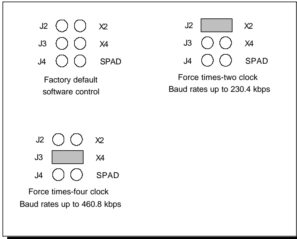
Figure 3 --- Clock multiplier jumper options
