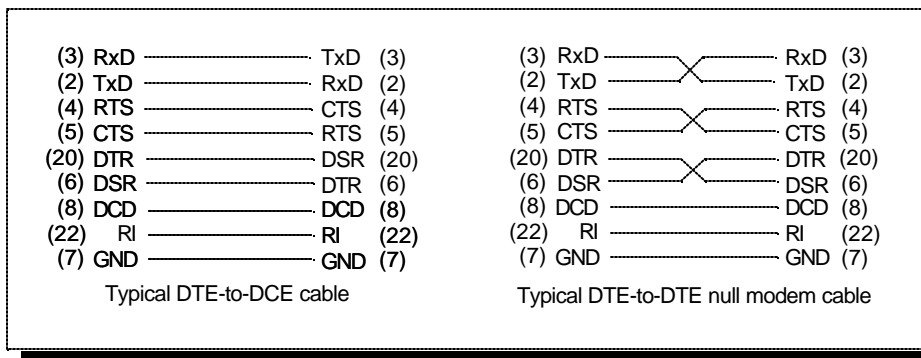
Figure 16 --- Cabling requirements for RS-232-C devices (cables using 25-pin connectors shown)
