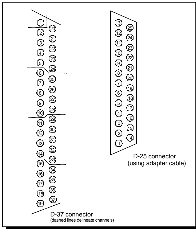
Figure 18 --- QSCP-100 output connectors
