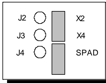
Figure 1 --- Factory default jumper configuration
