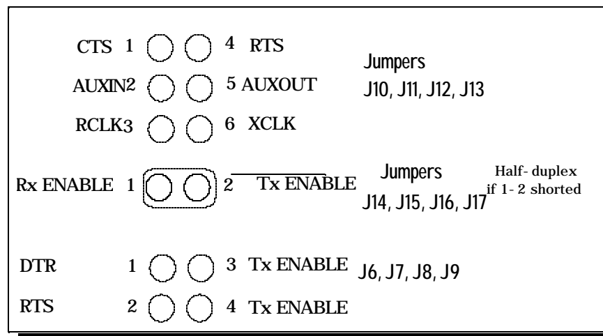
Figure 18 --- Pinout of jumpers J9-J16
