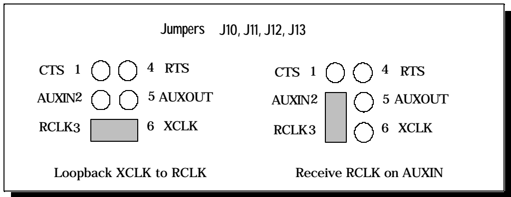
Figure 20 --- RCLK selection
