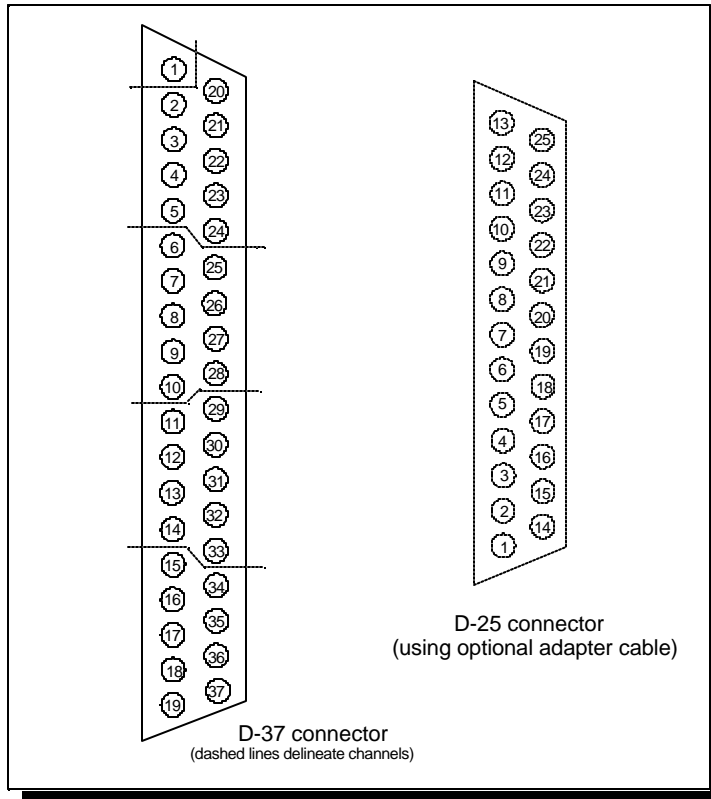
Figure 26 --- QSCP-200/300 connector definitions
