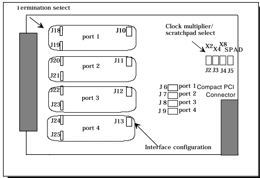
Figure 6 --- Jumper/connector locations
