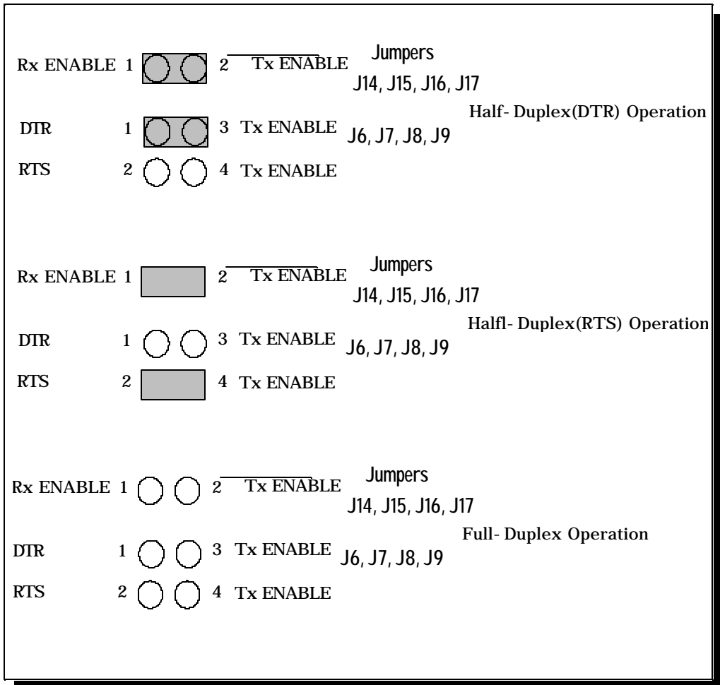
Figure 23 --- Half- or full-duplex selection
