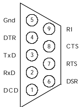
Figure 4. Standard D-9 male RS-232 connector signal assignment.
